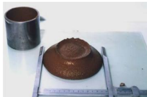
The flowability of sludge and/or stabilizer is measured using a flow ring with a dimension of \phi 77
